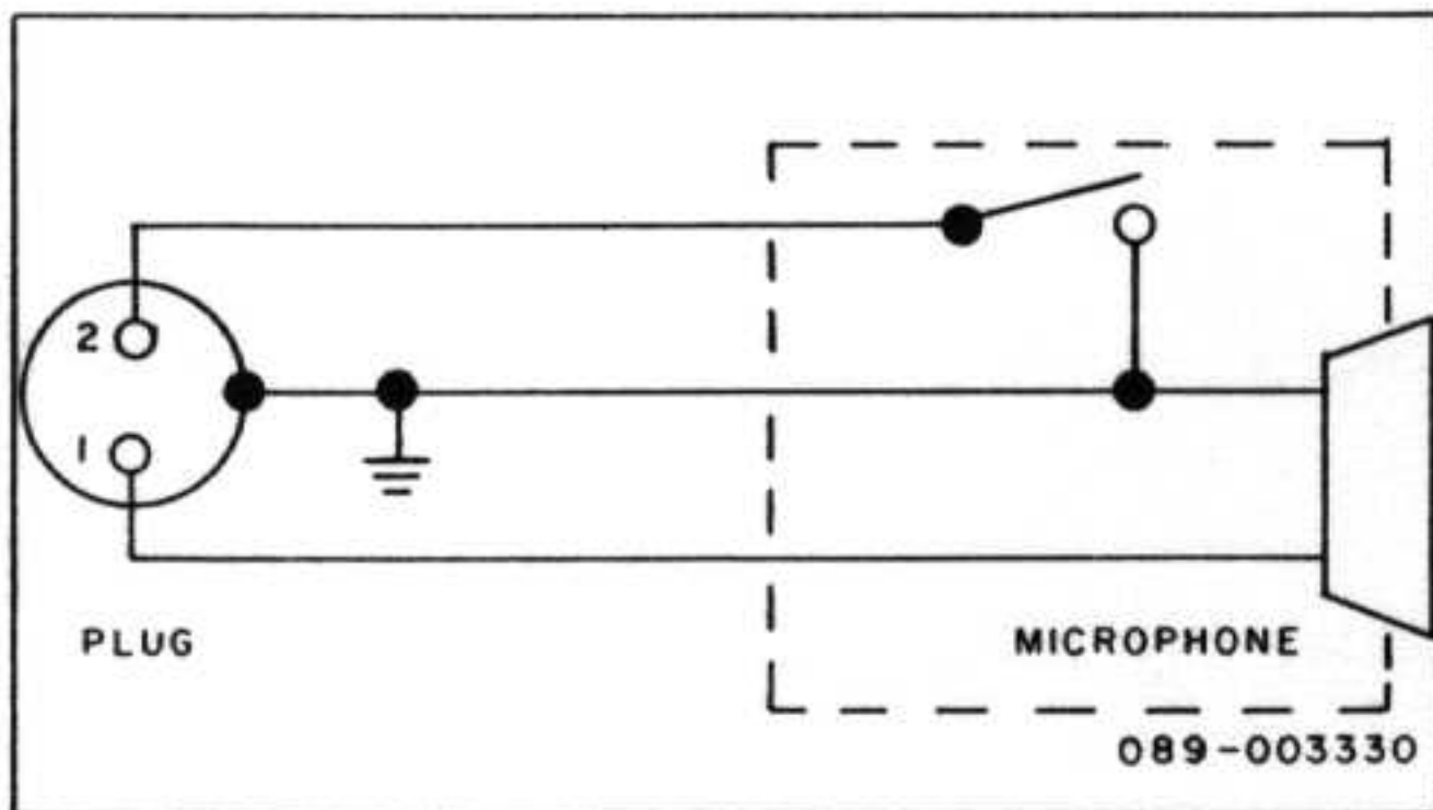
Figure 6. Required Microphone Wiring.
