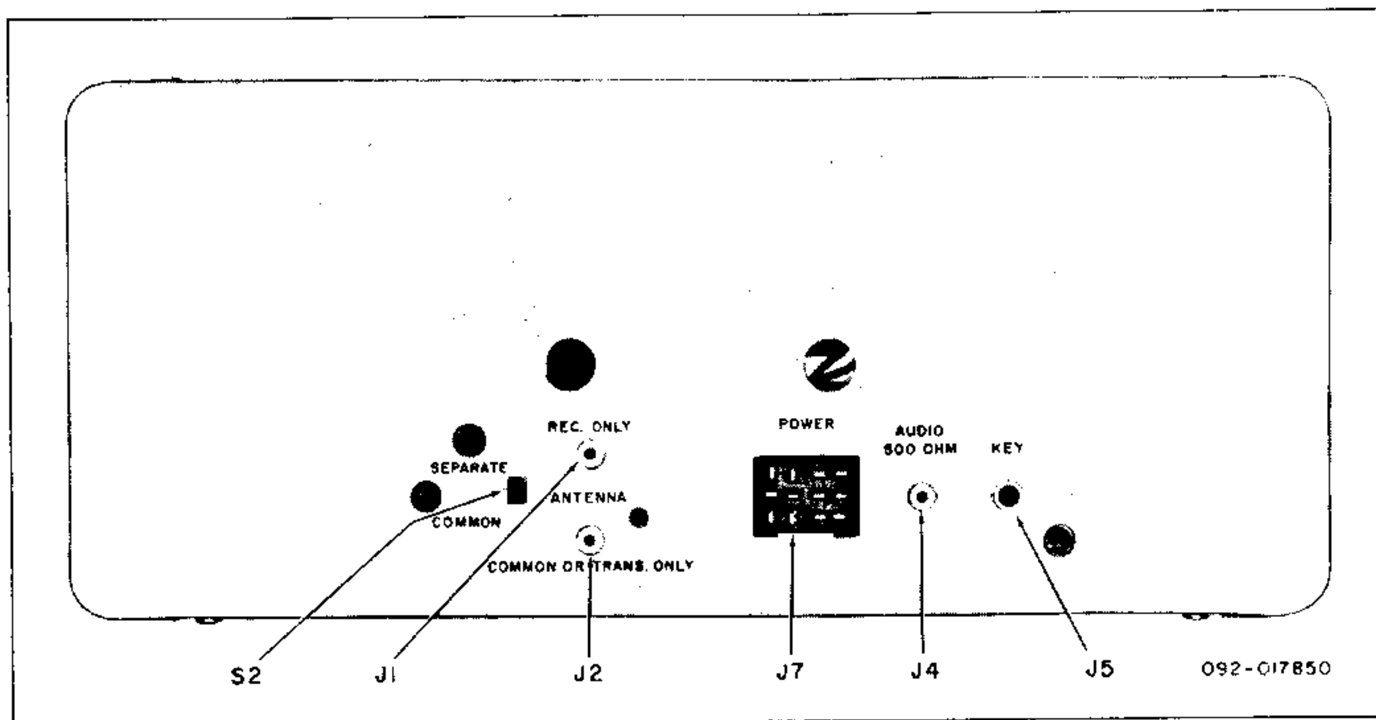
Figure 2. Rear View of Transceiver.
