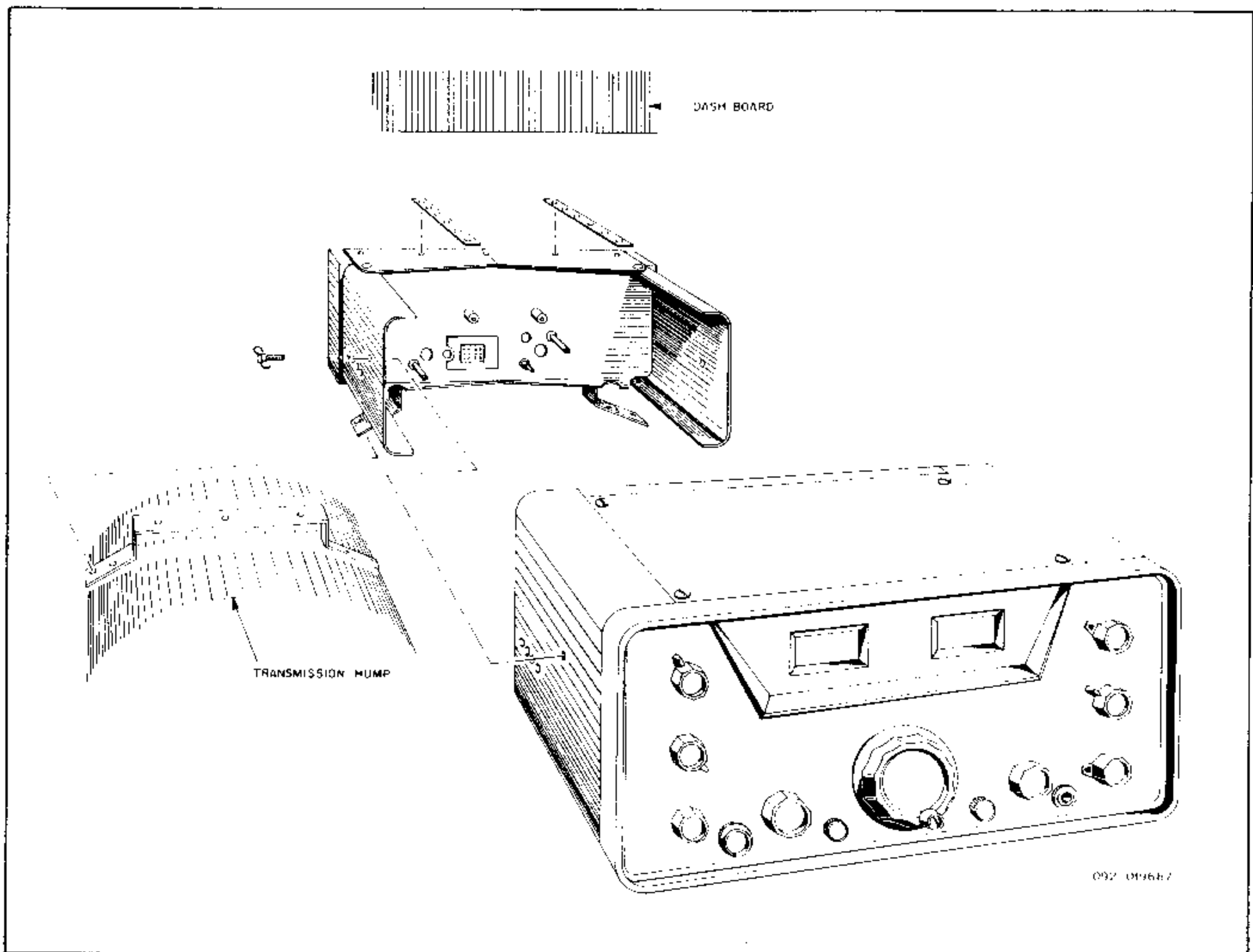
Figure 4. Installing the Model MR-150 Mounting Rack.
