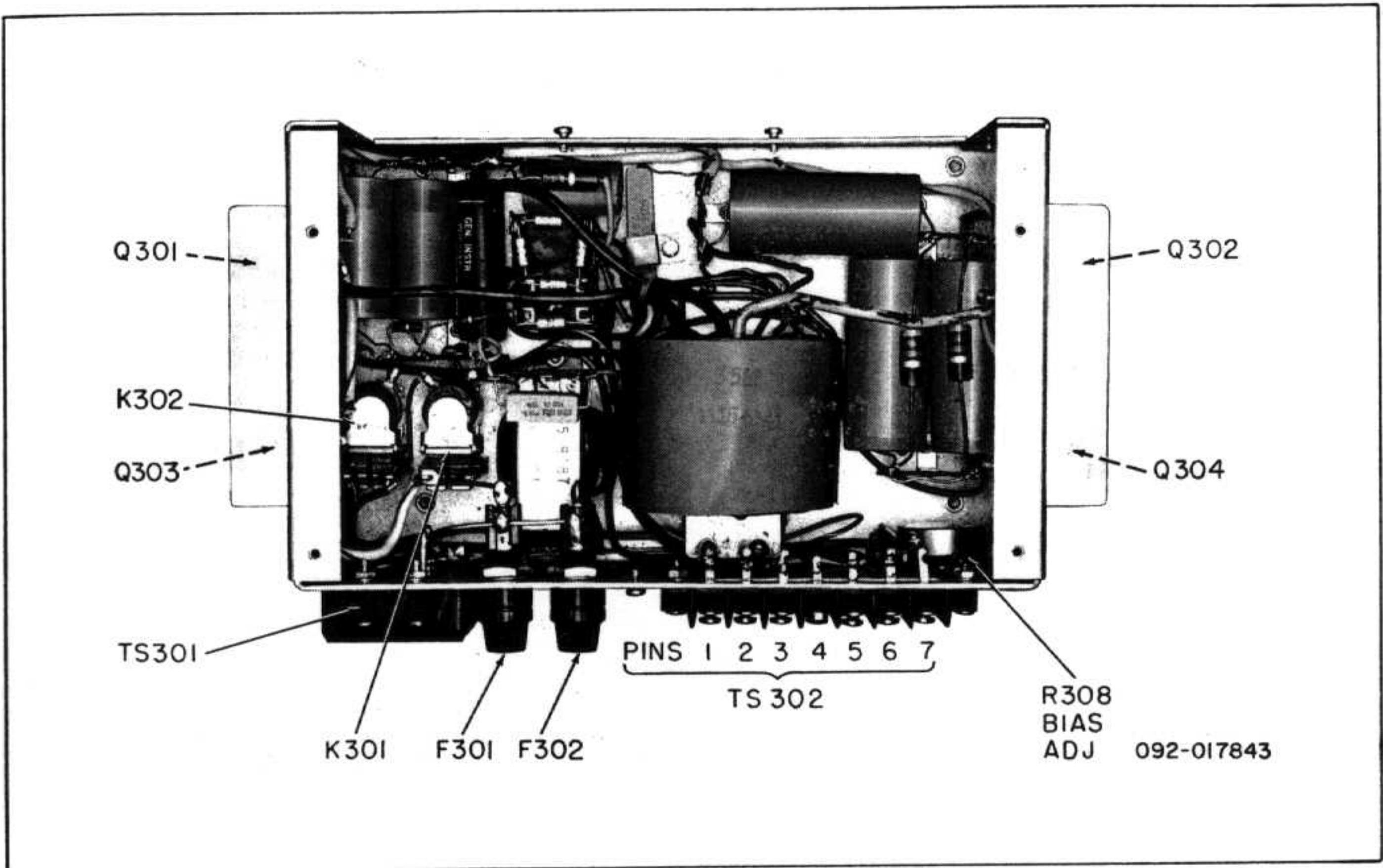
Figure 17. Internal Top View of Model PS-150-12 DC Power Supply.
