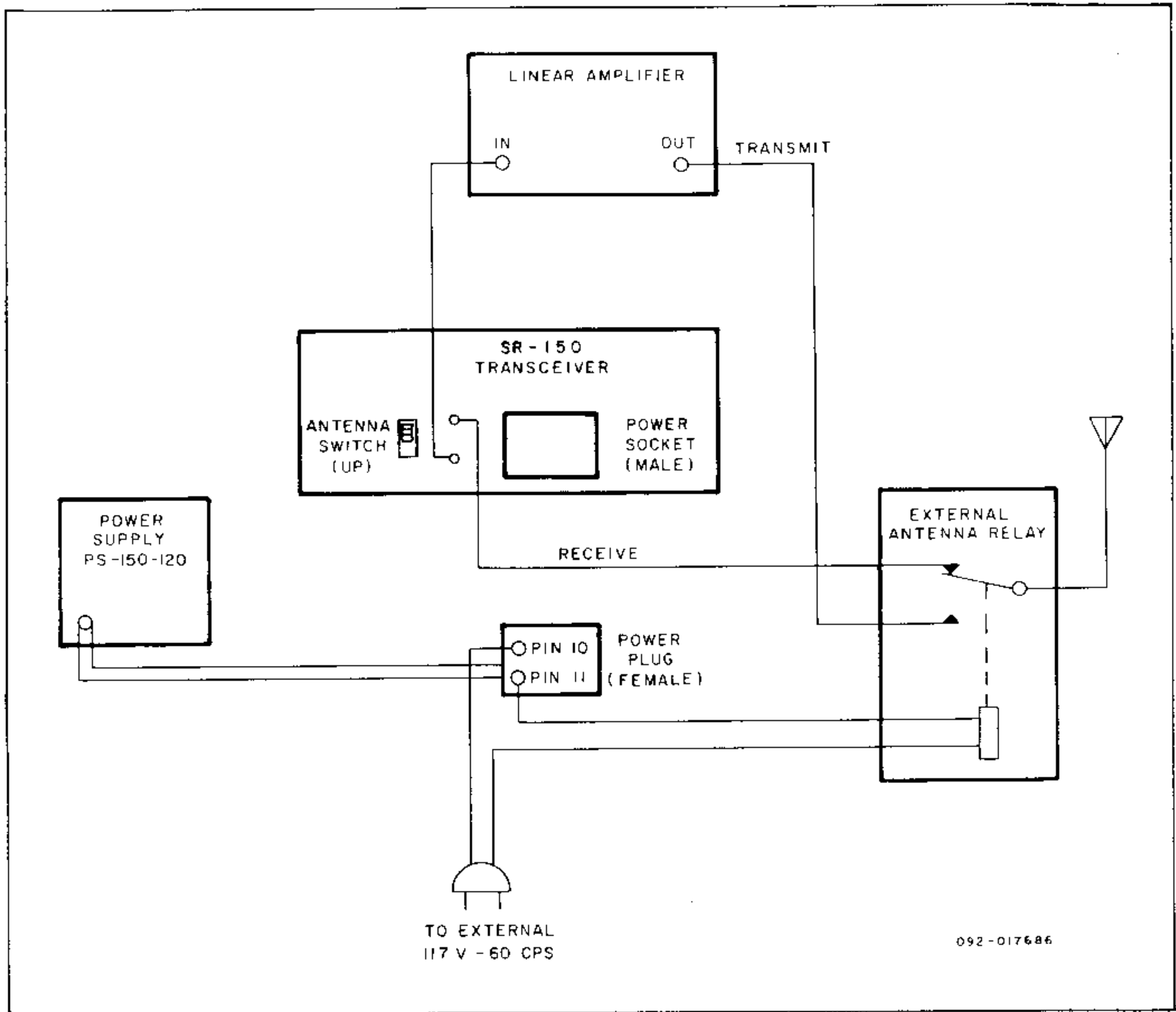
Figure 3. Base Installation Using a Linear Amplifier.
