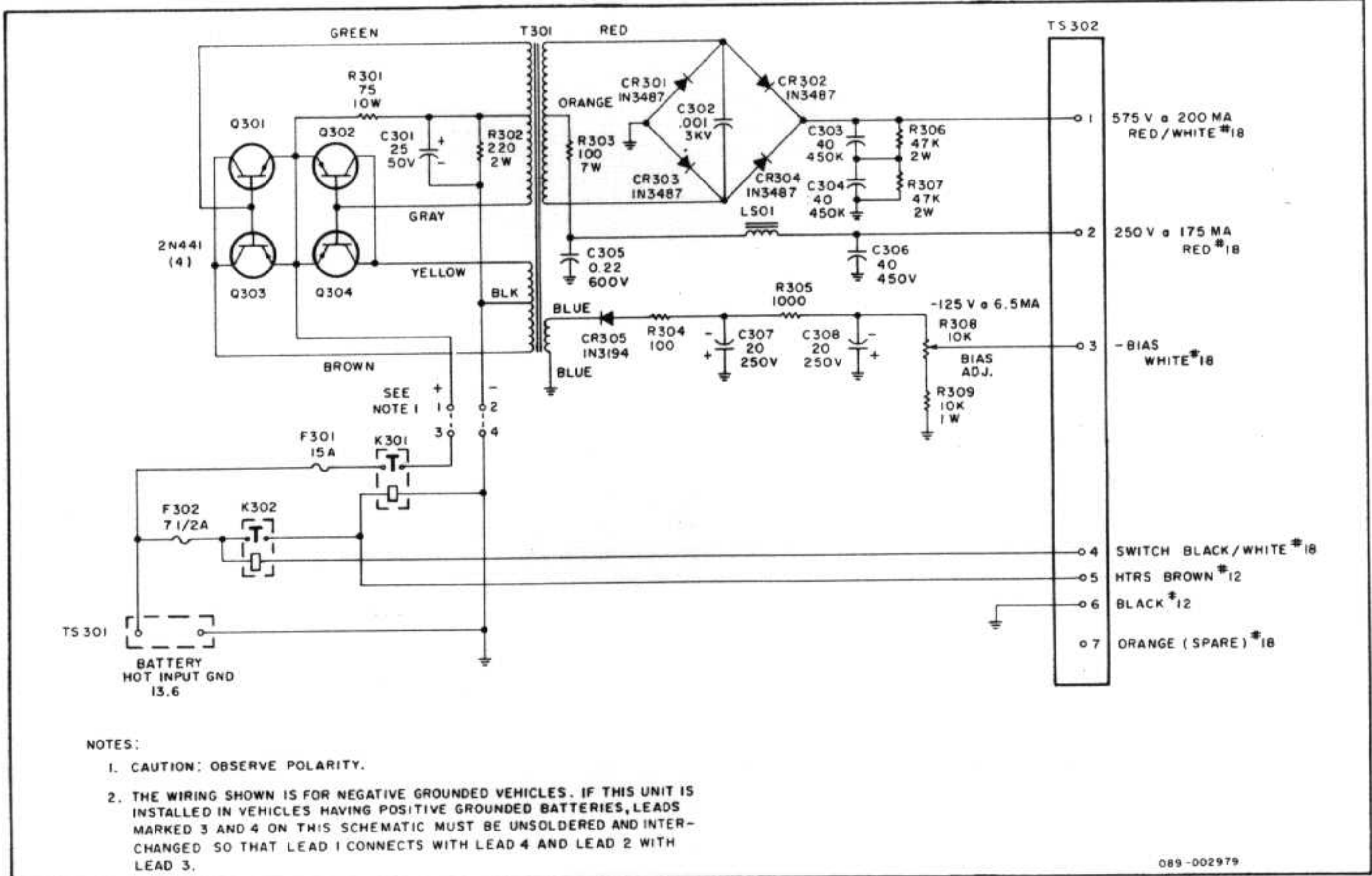
Figure 18. Schematic Diagram of Model PS-150-12 DC Power Supply.
