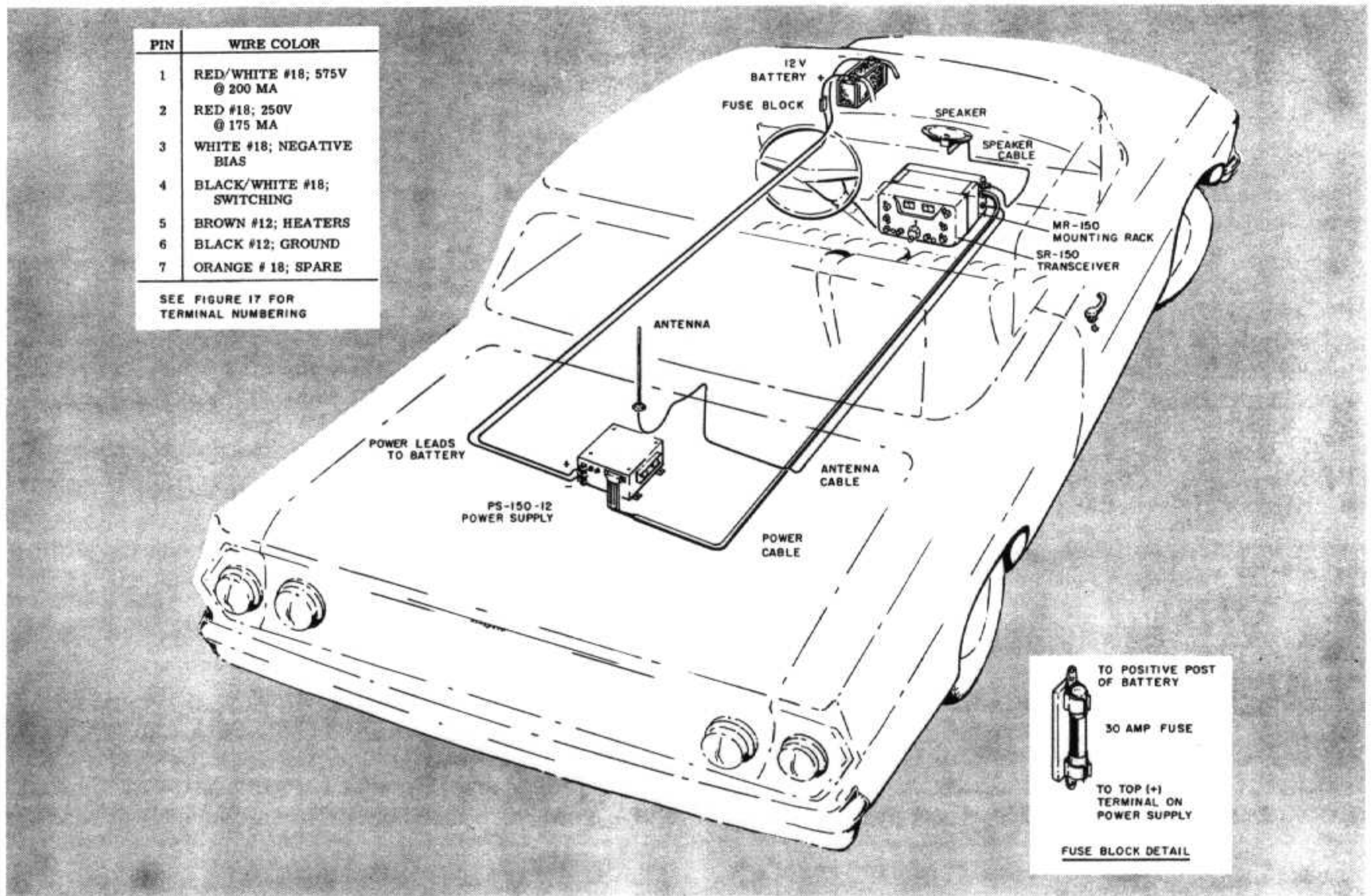
Figure 5. Wiring Diagram of Mobile Installation.
